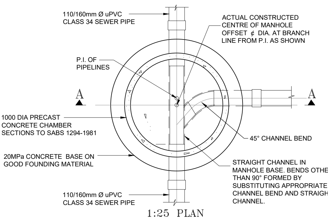
TYPICAL SEWER CONCRETE RING MANHOLE DETAIL
