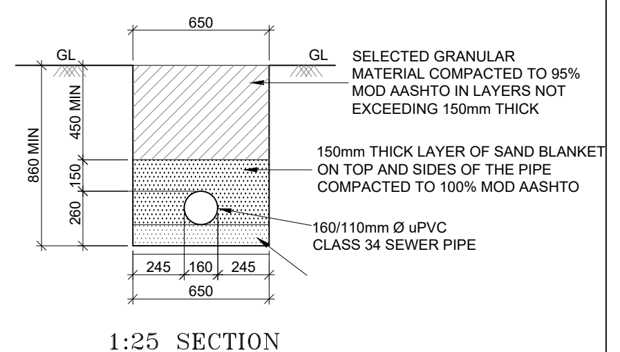
SEWER TRENCH
