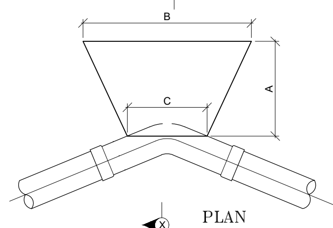
TYPICAL THRUST BLOCK DETAILS SCALE : NTS
