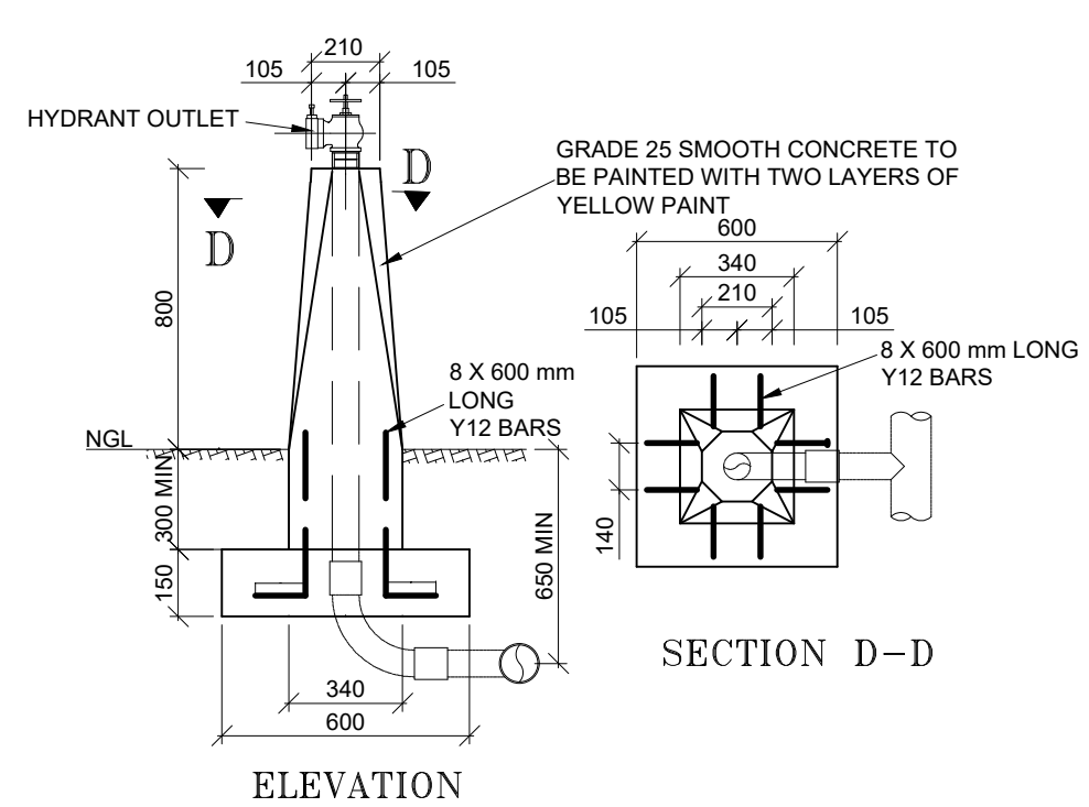
DETAILS OF ABOVE GROUND FIRE HYDRANTS SCALE : NTS
