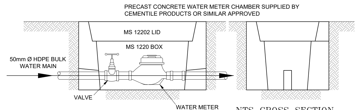
NTS LONG SECTION
